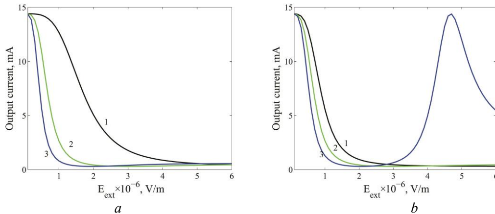
Figure – 2. Dependence of the signal on output of the resonators based on vertical slot waveguide with LC filling on electric field intensity. (a) Bend radius is equal to 32 μm, slot width is 100 (curve 1), 200 (2) and 300 (3) nm. (b) Slot width is equal to 200 nm, resonator radius is 16 (curve 1), 32 (2) and 64 (3) μm.
