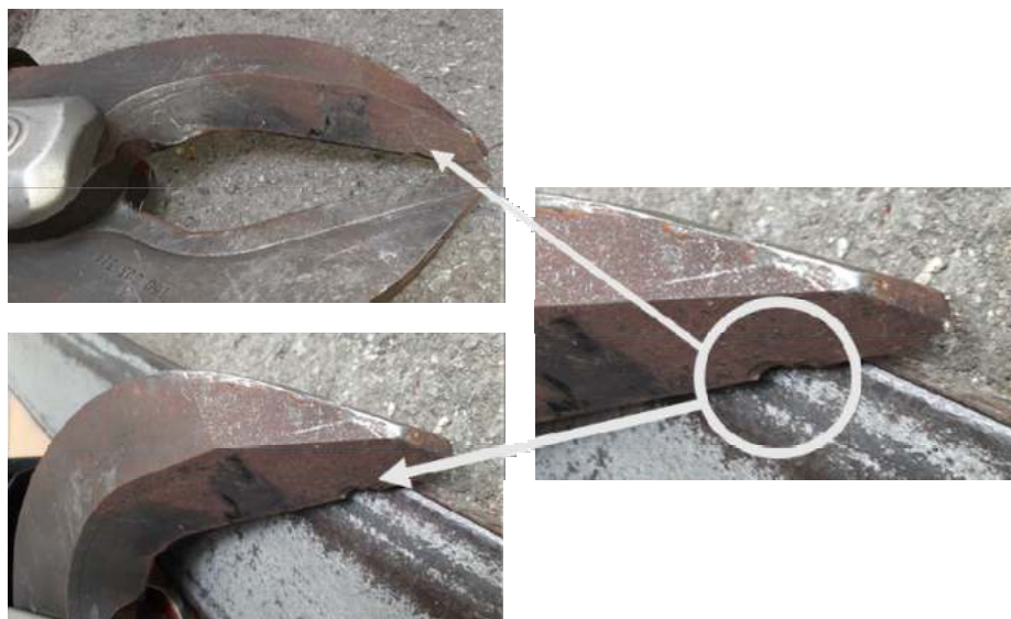
Photo1: cracks on the surface of emergecny equipment
